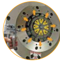
Easy grease maintenance through the 8 lubrication fittings
